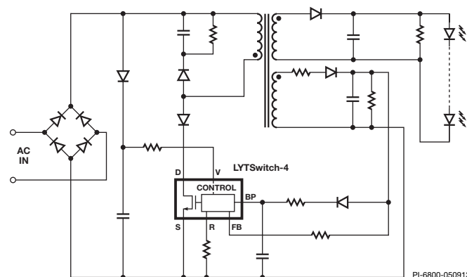
Figure 1. Typical Schematic.
